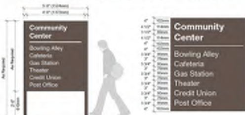
Figure 3-16 Centralized Facilities Freestanding Identification Signs.
