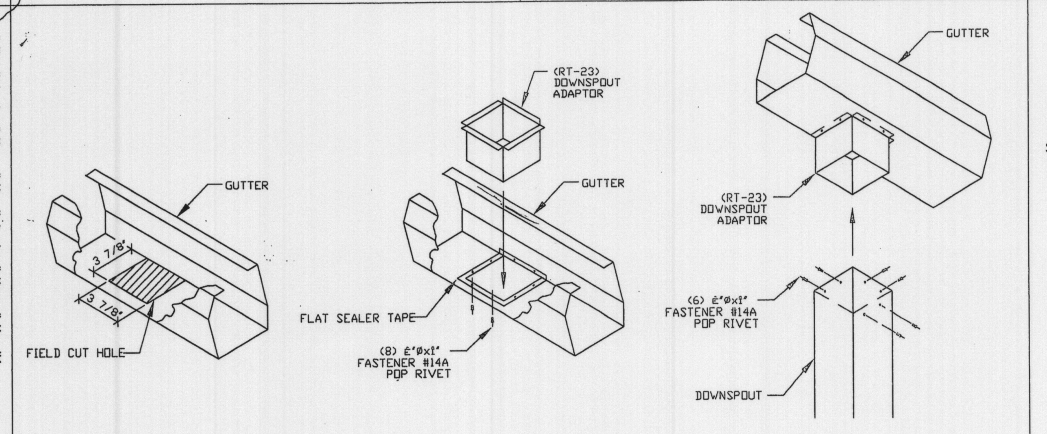
T16 DOWNSPOUT TO GUTTER
