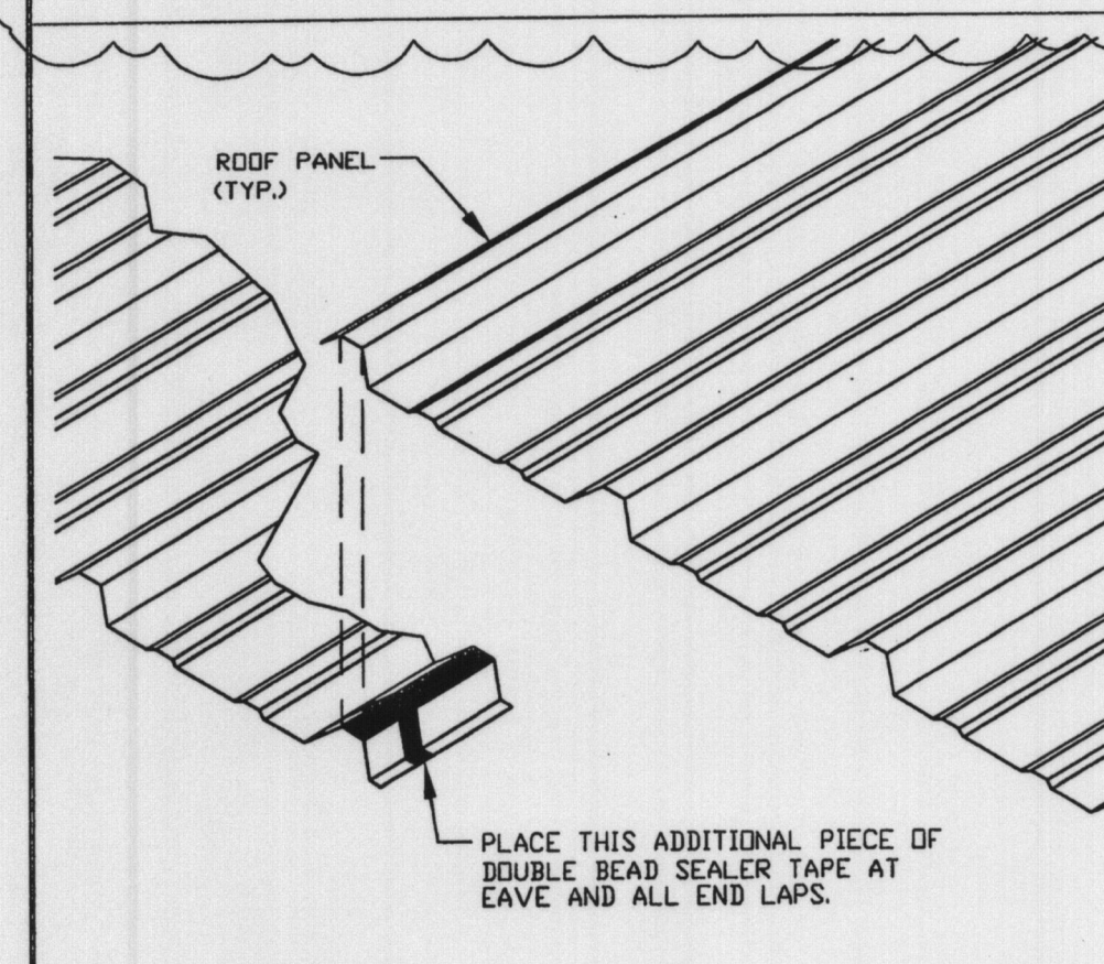
T15 SEALER TAPE AT EAVE SIDE
