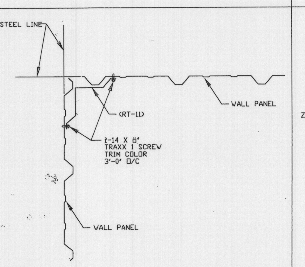
T7 INSIDE CORNER DETAIL
