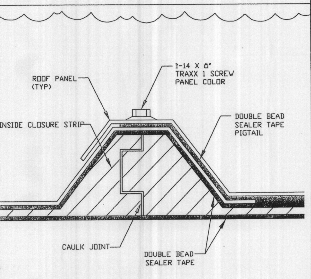
T14 SEALER TAPE/CLOSURE AT EAVE
