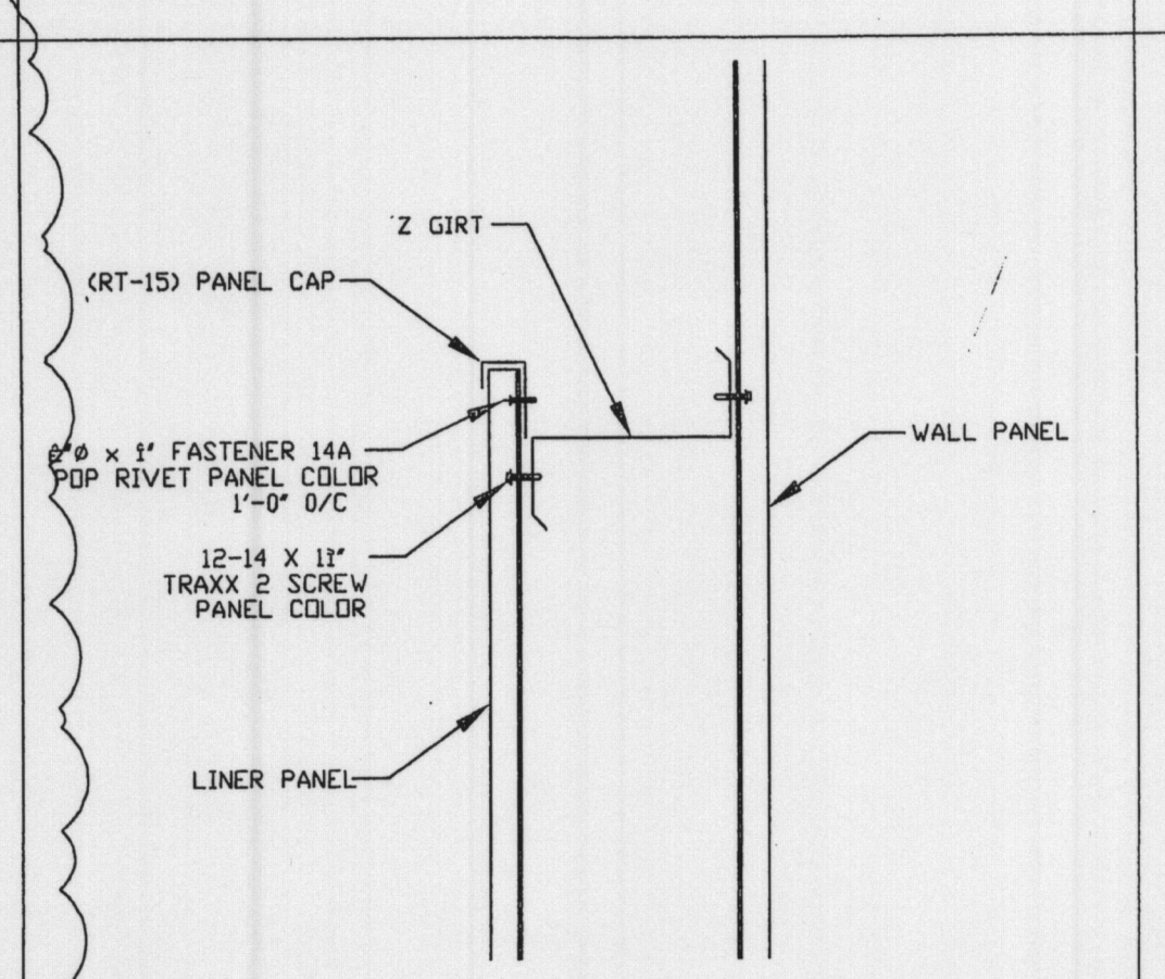
T11 LINER PANEL AT GIRT
