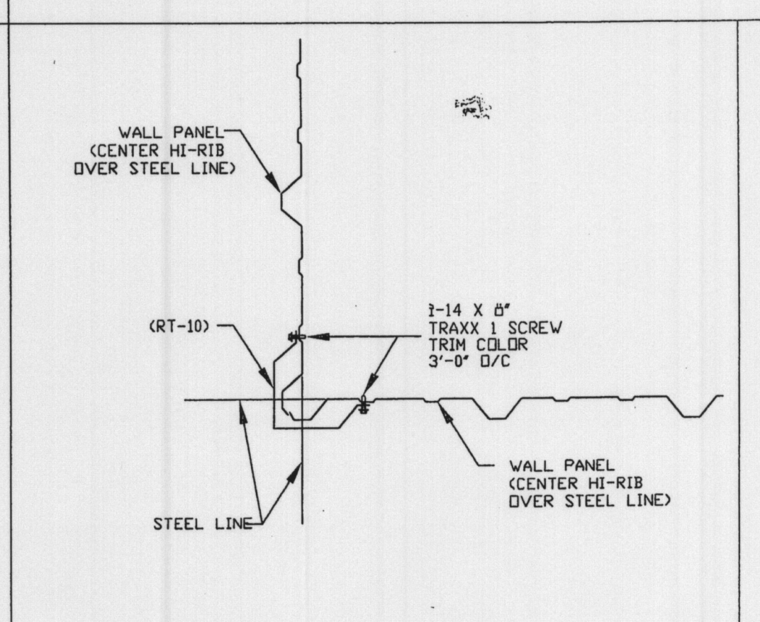
T6 OUTSIDE CORNER DETAIL
