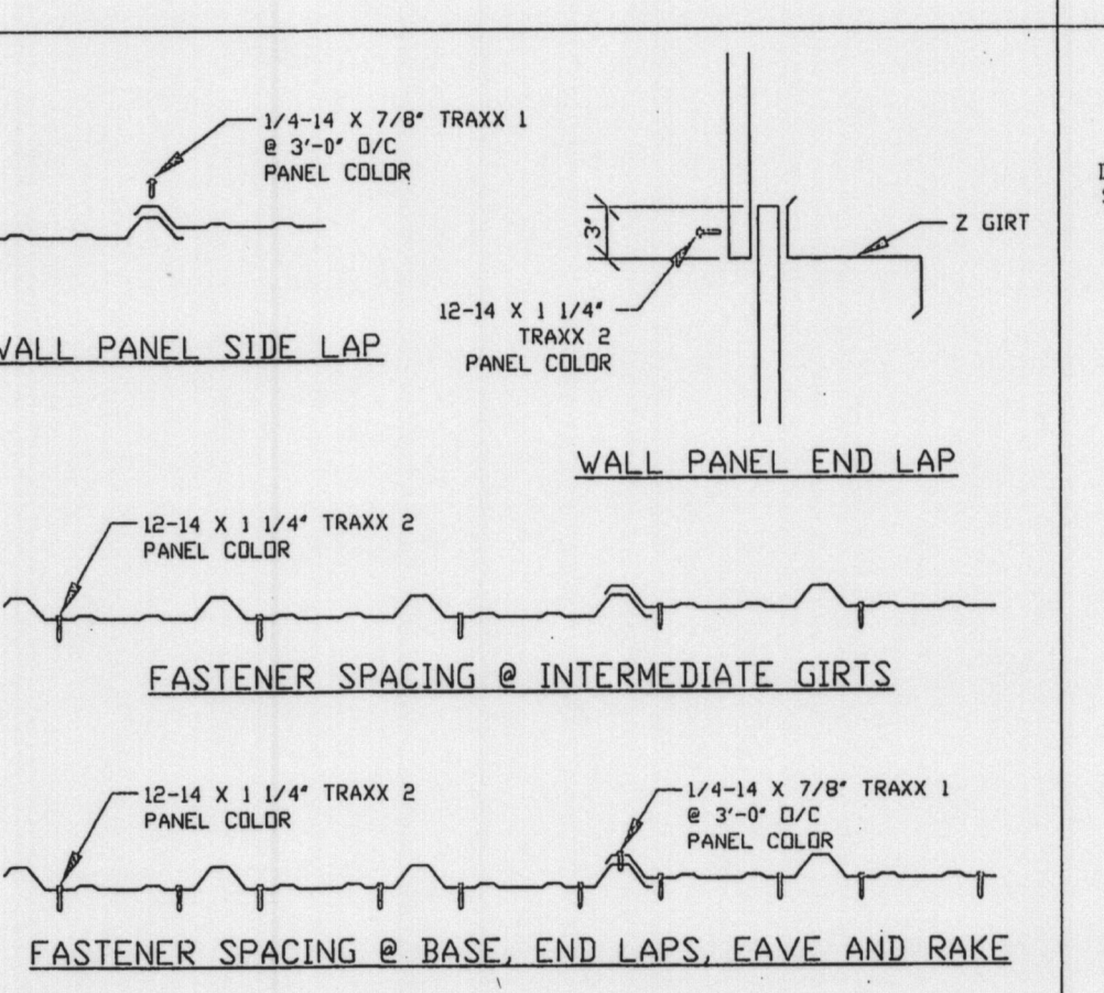
T12 WALL SCREWS
