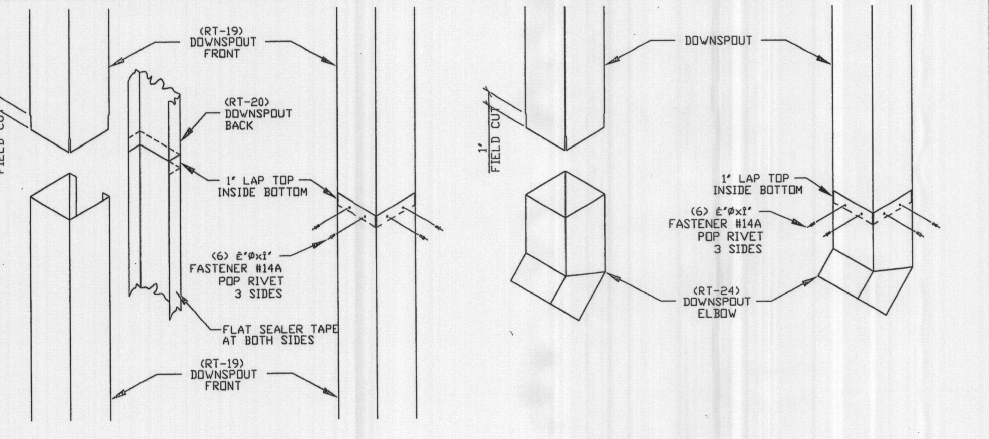
T17 2 PIECE DOWNSPOUT SPLICE & ELBOW
