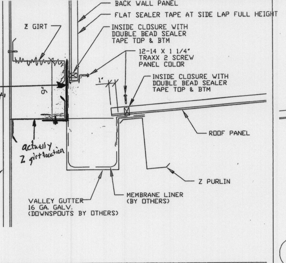
T4 WALL TO LOW ROOF
