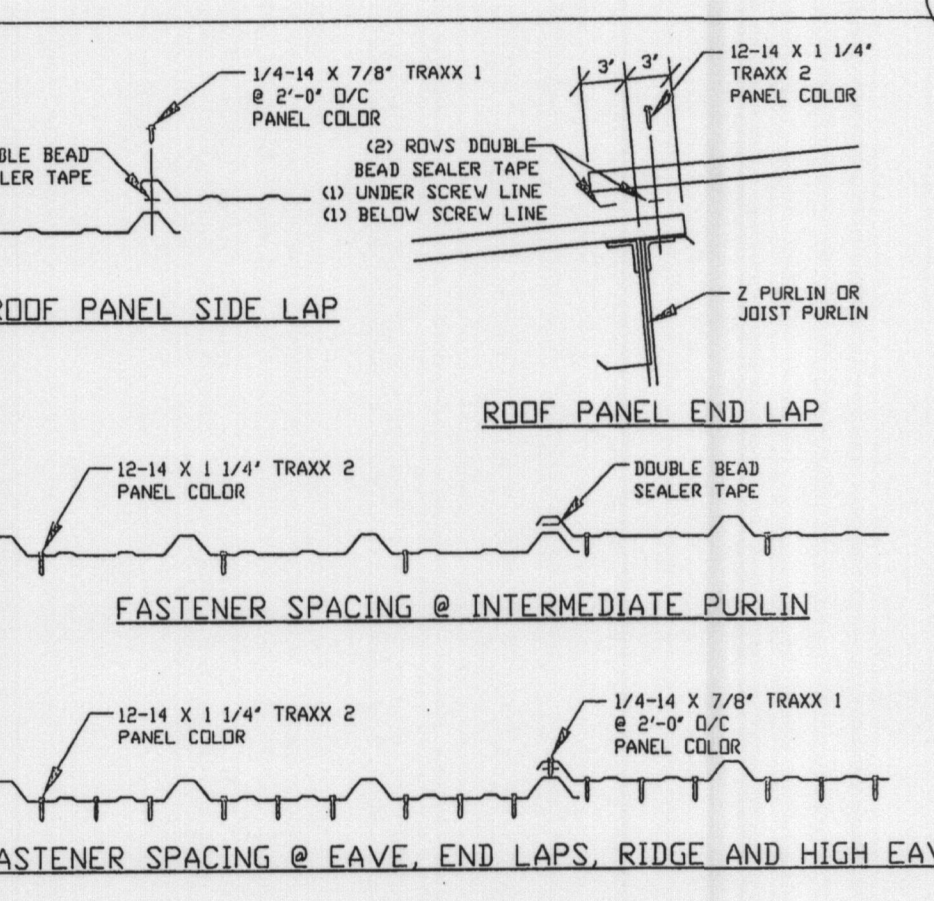
T13 ROOF SCREWS
