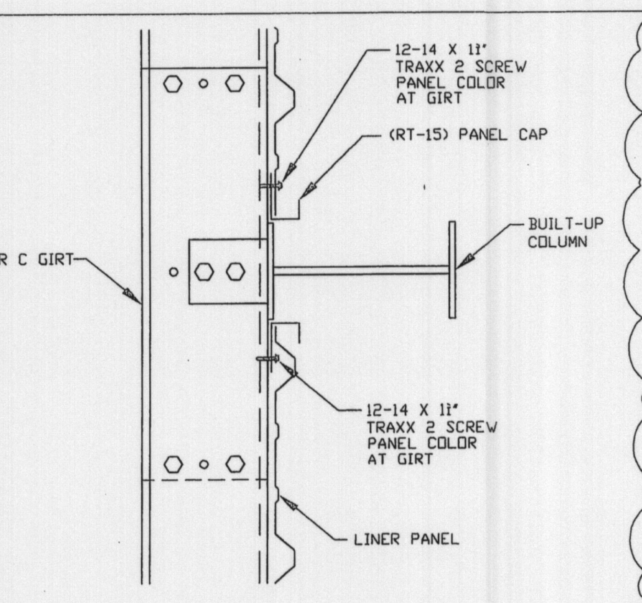
T8 LINER PANEL AT COLUMN
