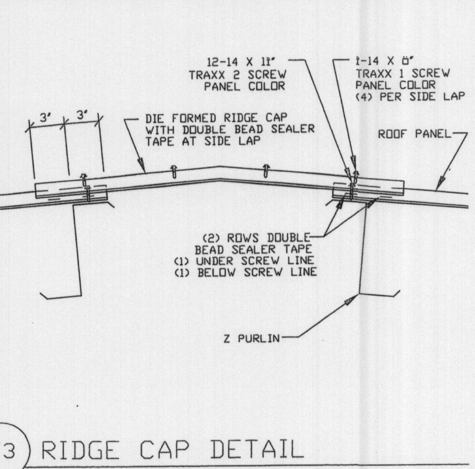
T3 RIDGE CAP DETAIL
