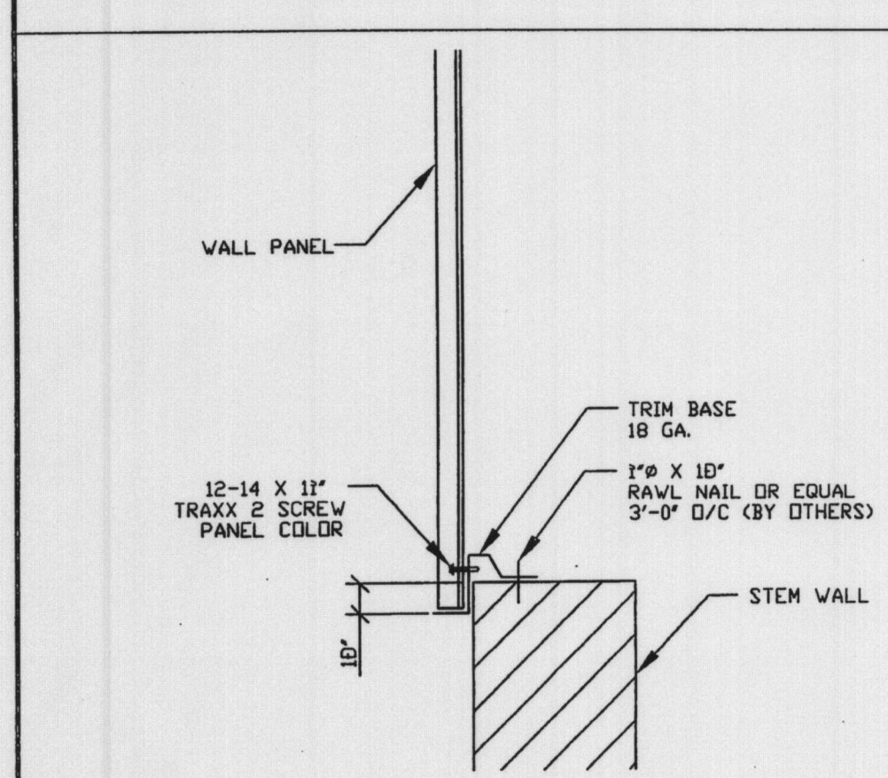
T5 PANEL BASE DETAIL
